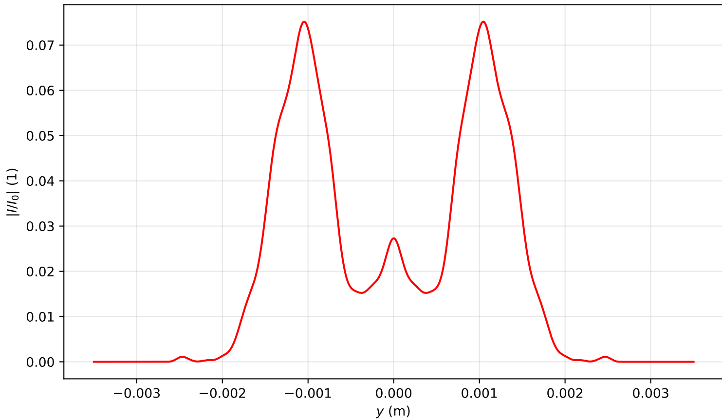
Intensity profile I(x=0, y, z=3.105)/I_0 , P_{in}=6.5P_{cr} , artificial time
